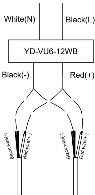
FACTORY CONNECTIONS (+) INNER CONDUCTOR | OUTER MESH (-)
