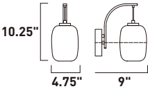
E25061-92BKGLD Wall Mount
