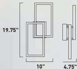
E21511-BK Outdoor Wall Mount Suitable for Wet Location C
