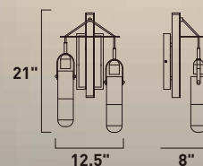
E24172-93BKAL Wall Mount
