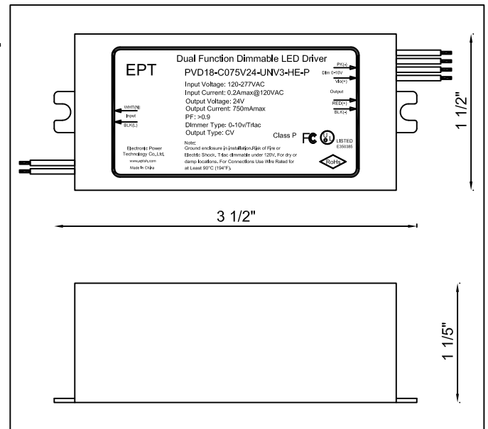
LED DRIVER DIAGRAM
