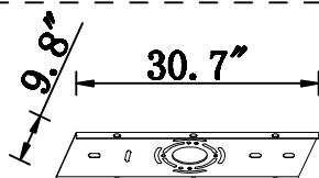
Mounting Bracket
