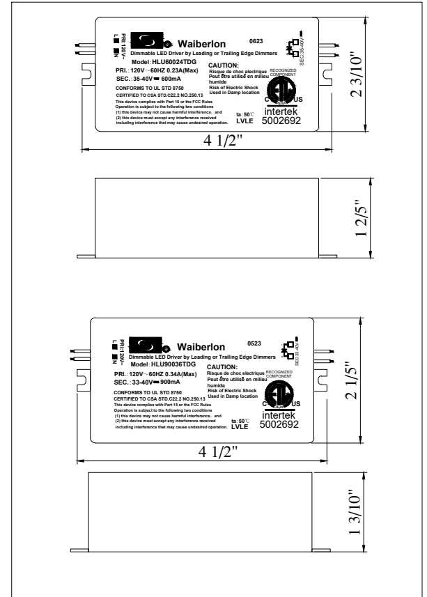
LED DRIVER DIAGRAM
