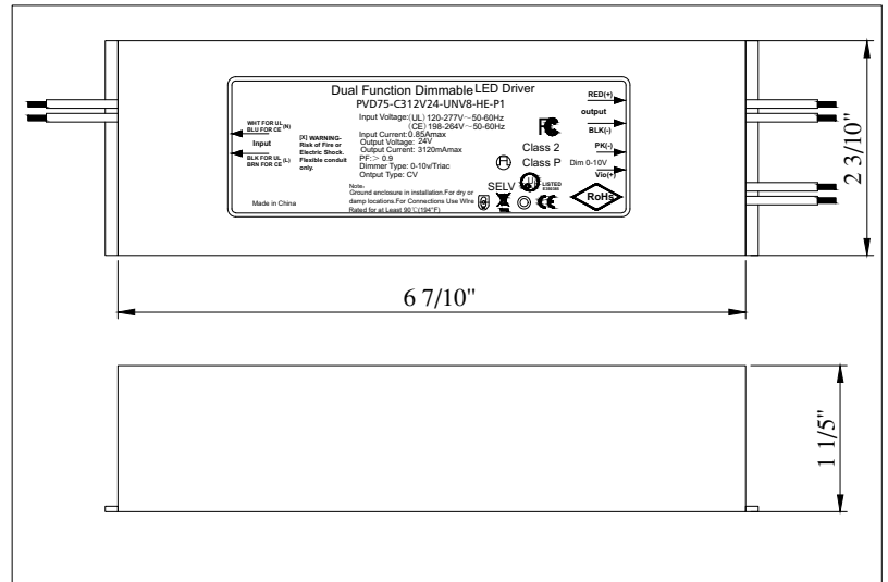
LED DRIVER DIAGRAM
