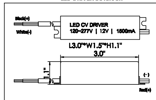
LED DRIVER DIAGRAM
