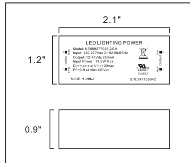
LED DRIVER DIAGRAM
